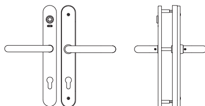
Model E1012 Electronic Escutcheon E1000 Comfort iButton. 2 Handles, any type. Inside/Outside Cylinder outtake. With connector for Mortise Lock with Micro-Switch.
