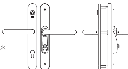
Model E1017 Electronic Escutcheon E1000 Comfort iButton. 2 Handles, any type. Electronic "Do not disturb" system. Outside Cylinder outtake.
