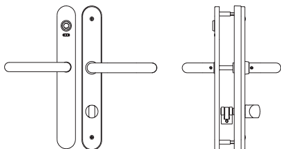
Model E1011 Electronic Escutcheon E1000 Comfort iButton. 2 Handles, any type. Inside Thumbturn. With connector for Mortise Lock with Micro-Switch.
