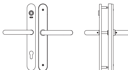
Model E1014 Electronic Escutcheon E1000 Comfort iButton. 2 Handles, any type. Outside Cylinder outtake.
